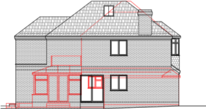
PROPOSED LEFT SIDE ELEVATION
