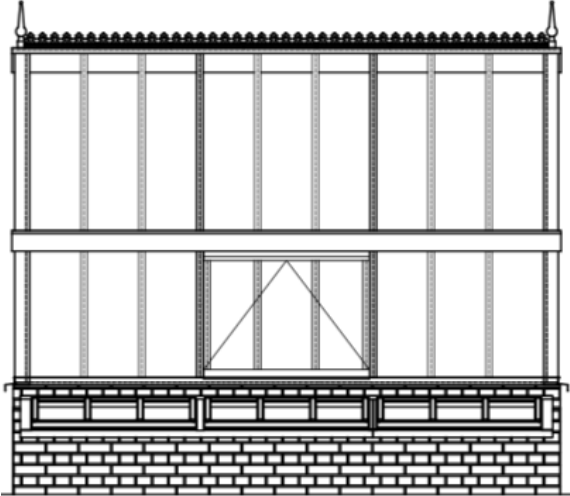
3744mm RIGHT ELEVATION
