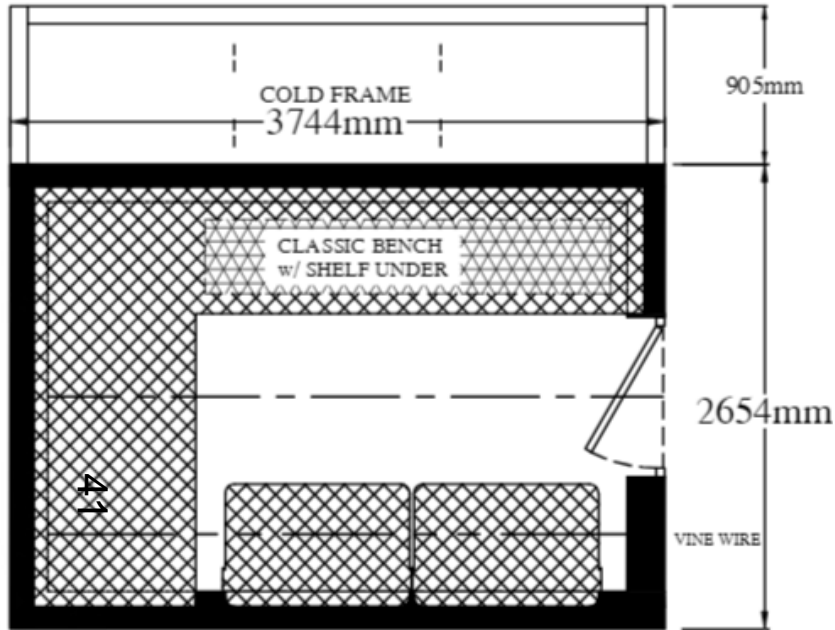
FLOOR PLAN
