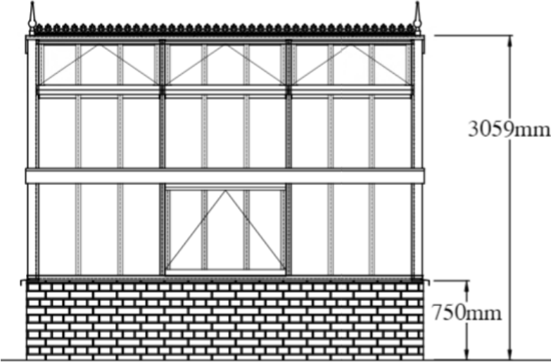
3744mm LEFT ELEVATION
