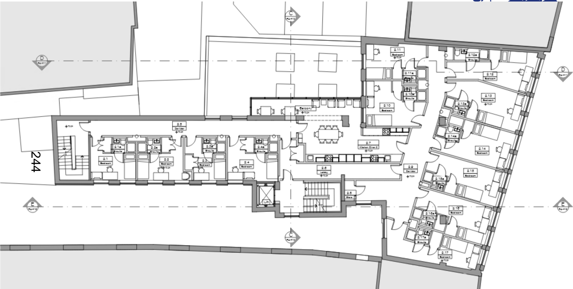
2 SECOND FLOOR PLAN 1:100
