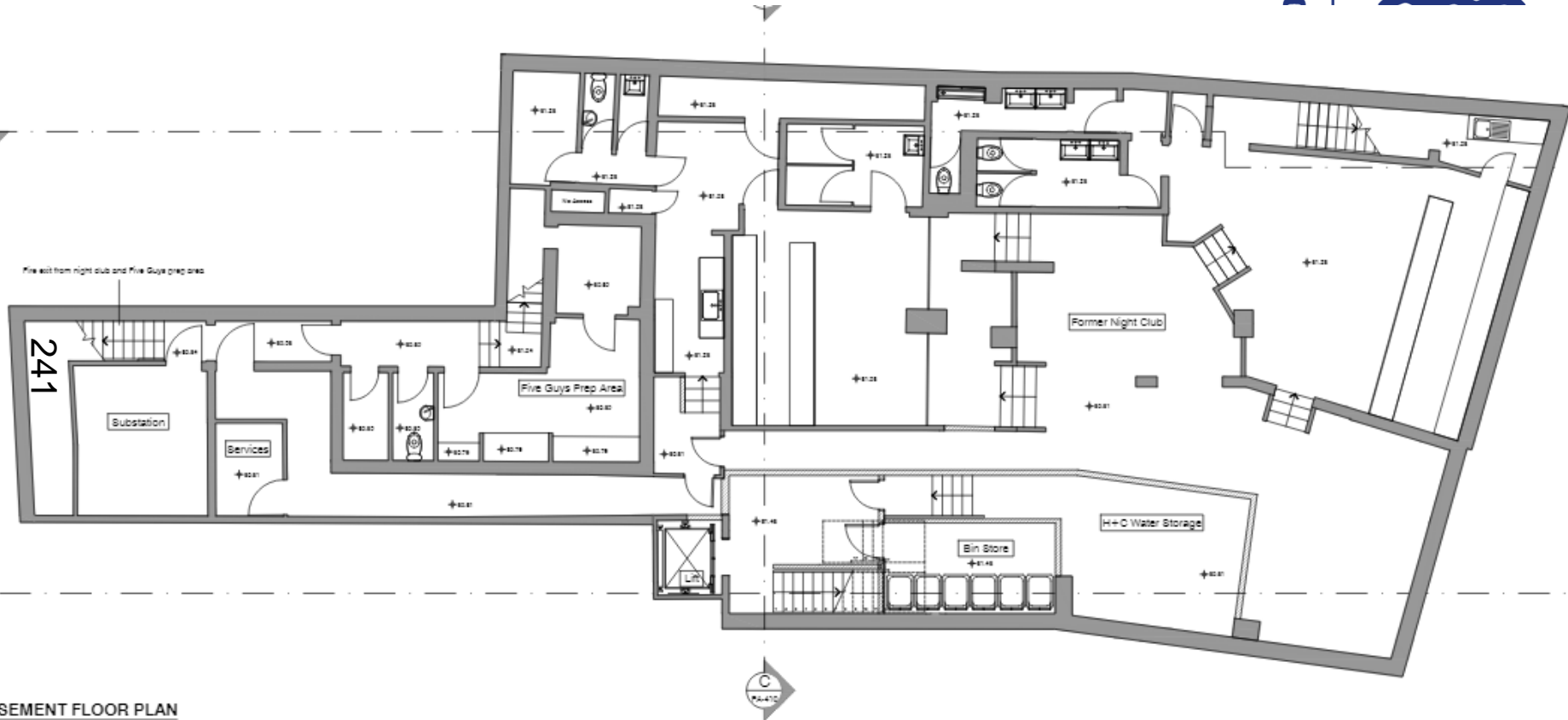
BASEMENT FLOOR PLAN 1:100
