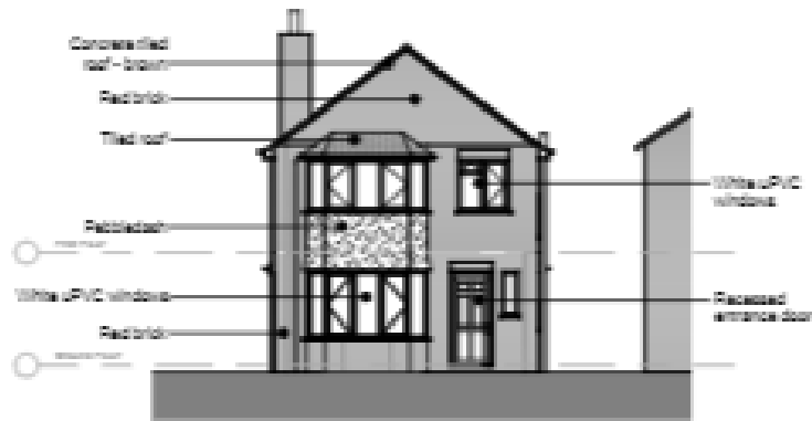
4 North-East (Front) Elevation. 1 : 100
