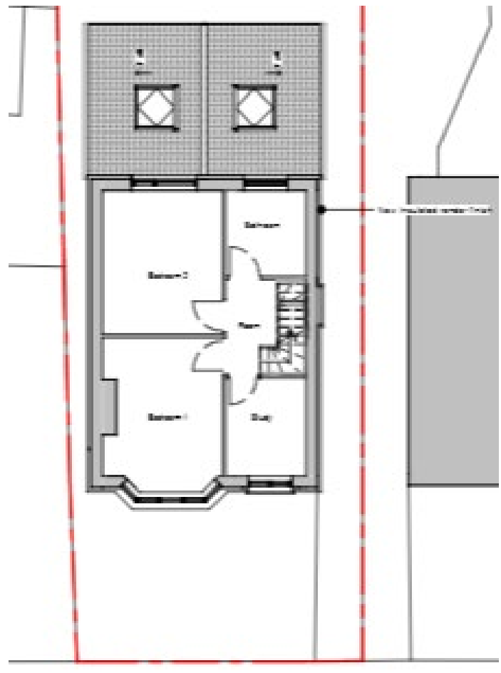
2 First Floor Plan - Proposed
