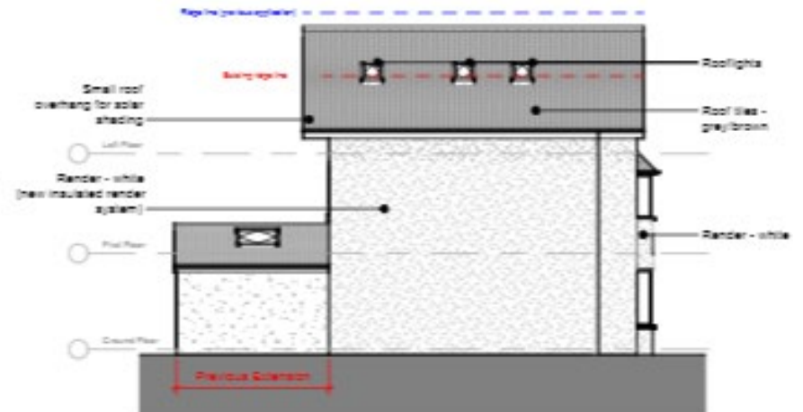
8 South-East Elevation - Proposed
