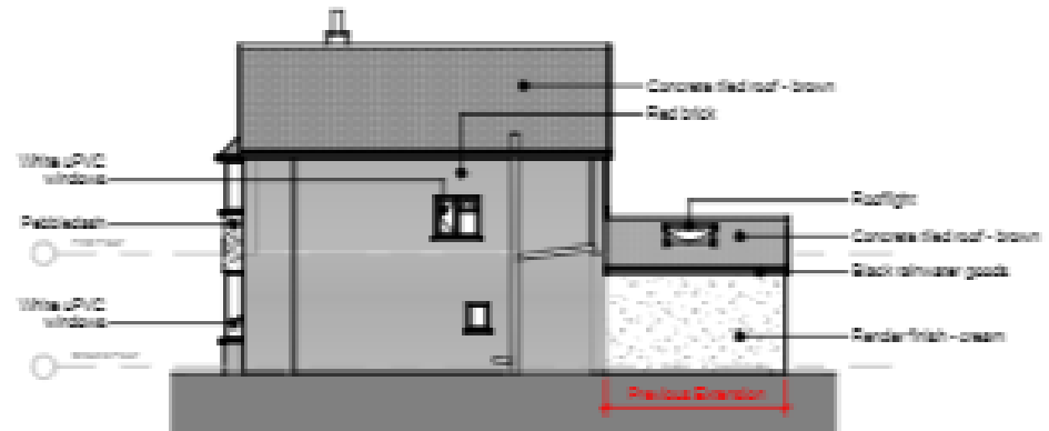
5 North-West Elevation. 1 : 100
