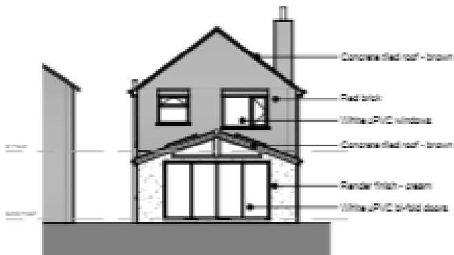
6 South-West Elevation. 1 : 100
