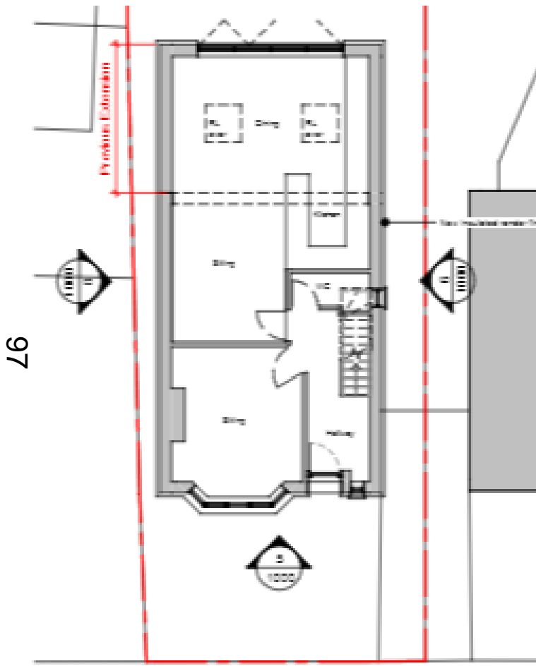
1 Ground Floor Plan - Proposed
