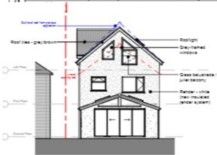
5 North-East (Front) Elevation - Proposed
