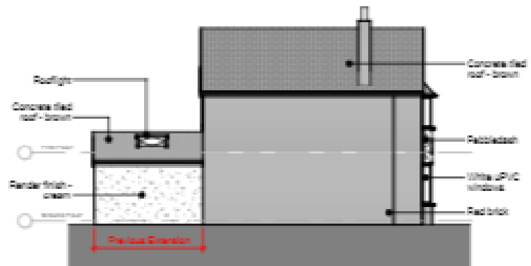
7 South-East Elevation. 1 : 100
