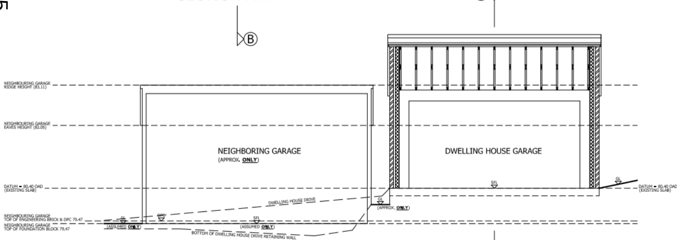
SECTION B-B
