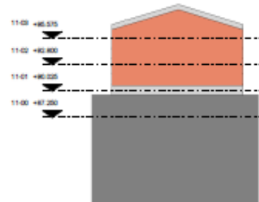
2 East Elevation 1:50
