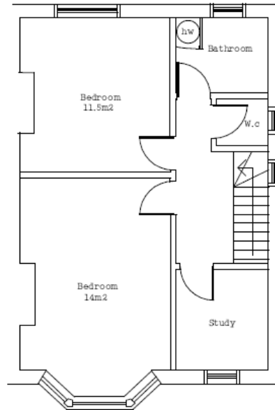
Proposed 1st floor
