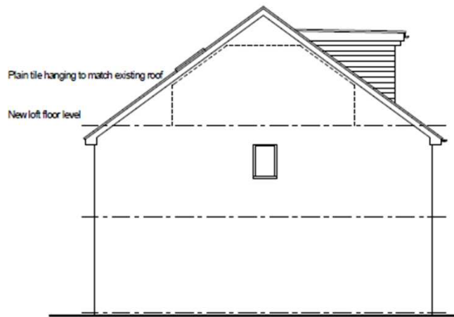
Side (North-West) Elevation Similar Side (North-East) Elevation
