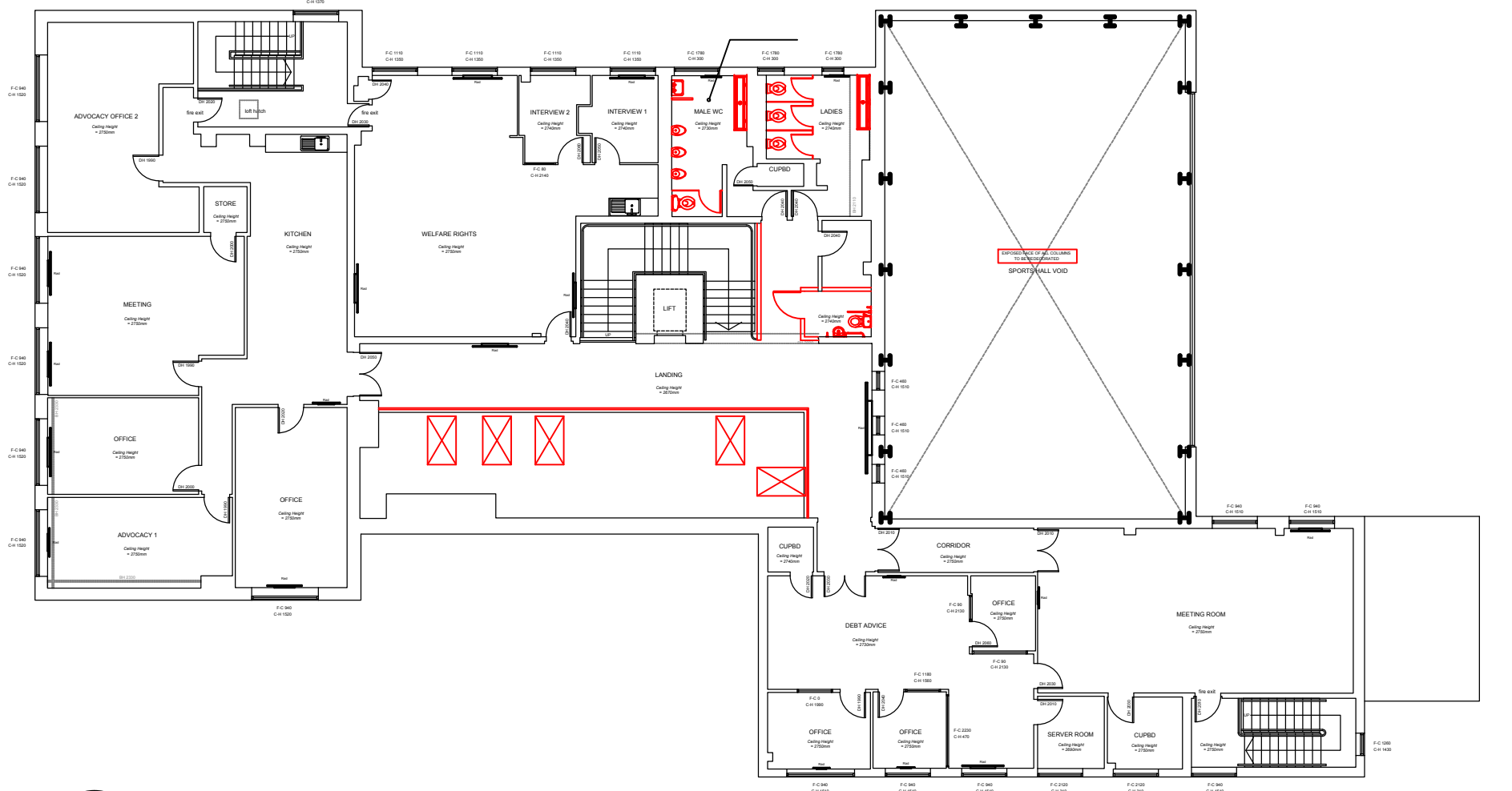
02 PROPOSED FIRST FLOOR P03 / 1:200 scale@A1 size
